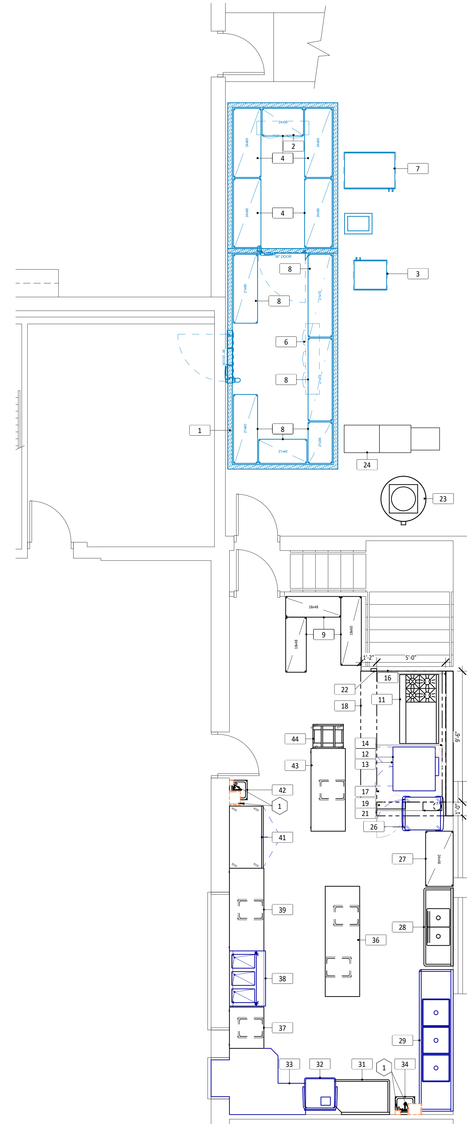
1 FOODSERVICE EQUIPMENT PLAN FS101 1/4" = 1'-0"
